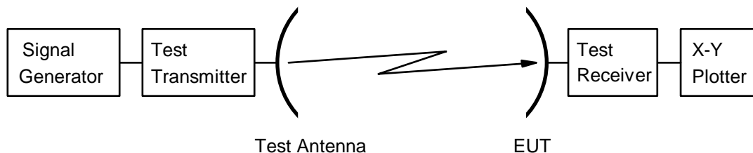
Figure 13: Test arrangement - antenna transmit radiation pattern measurement
