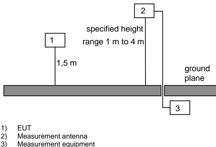
Figure E.1: Measurement arrangement
