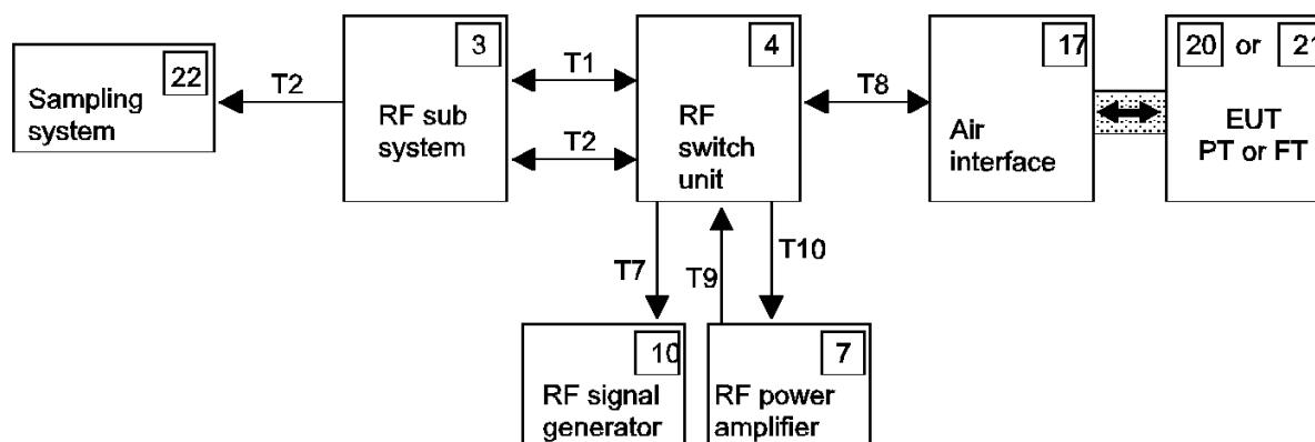
Figure 22: Test setup 5
