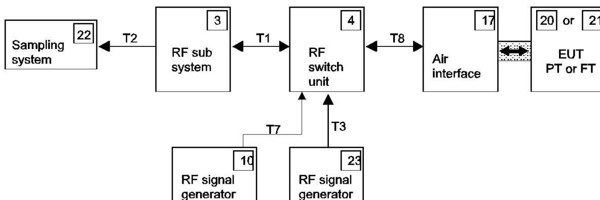
Figure 20: Test setup 3
