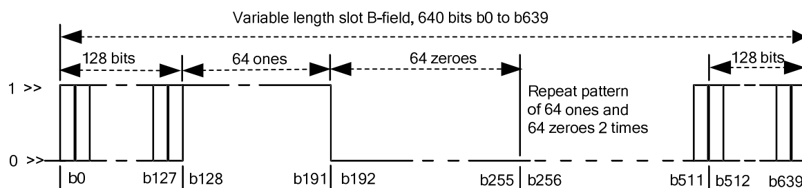
Figure 37: Test packet transmission for case 2, full-slot
