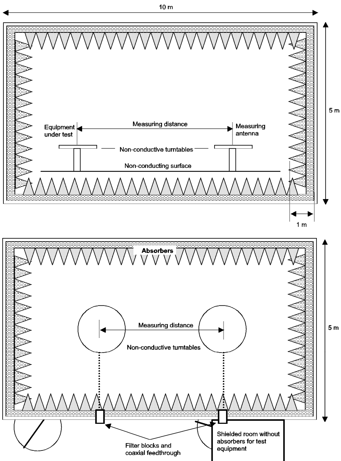
Figure 13: Construction example
