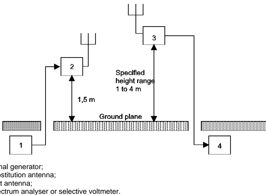
Figure B.4: Measurement arrangement No.2
