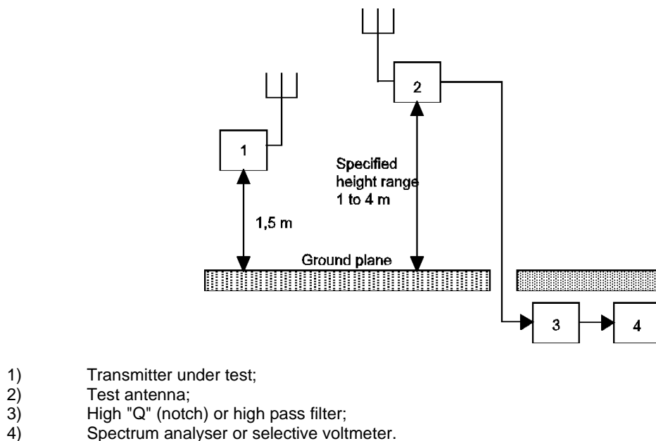
Figure B.3: Measurement arrangement No.1
