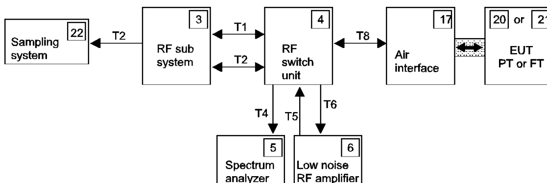
Figure 21: Test setup 4
