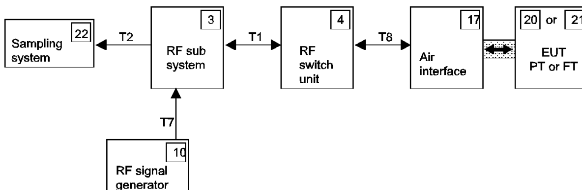
Figure 19: Test setup 2
