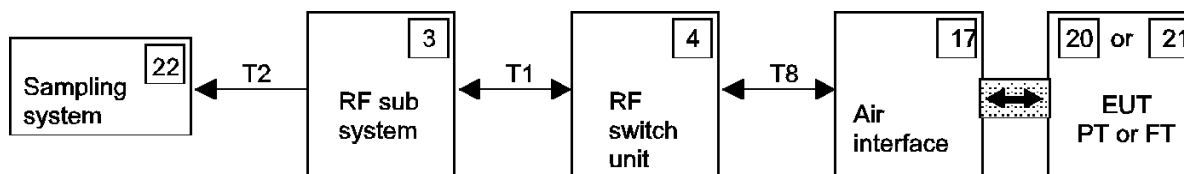
Figure 18: Test setup 1
