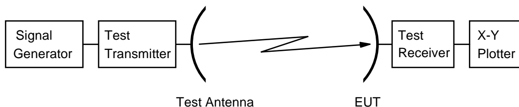
Figure 13: Test arrangement - antenna receive pattern measurement
