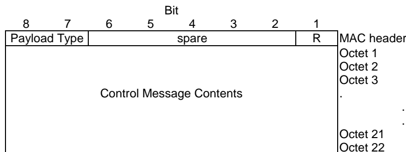
Figure 9: Uplink RLC/MAC control block together with its MAC header
