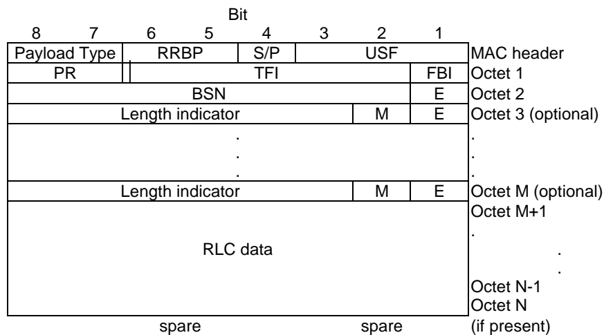
Figure 6: Downlink RLC data block with MAC header
