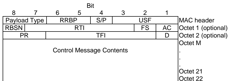
Figure 8: Downlink RLC/MAC control block together with its MAC header
