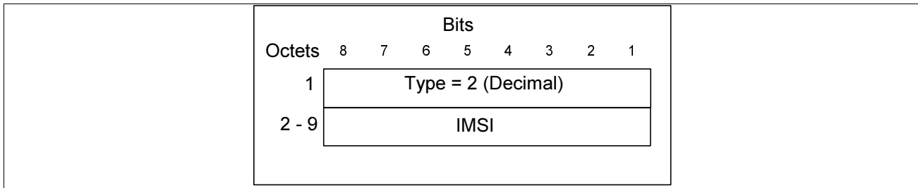
Figure 9: IMSI information element
