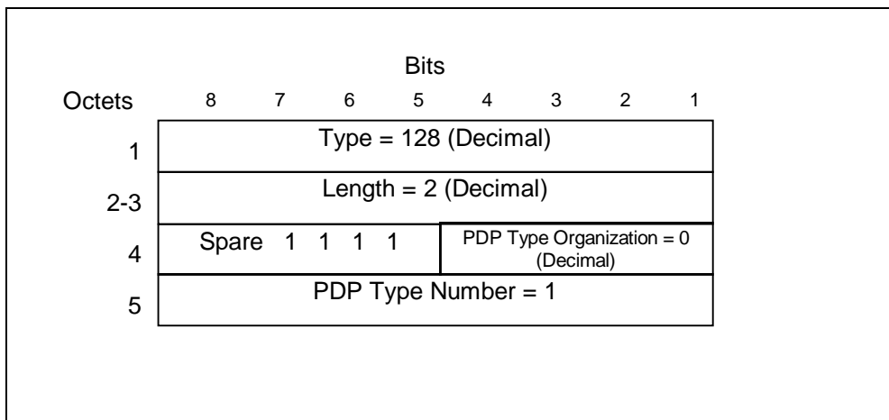
Figure 30: End User Address information element for X.25
