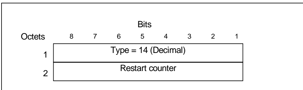
Figure 21: Restart counter information element
