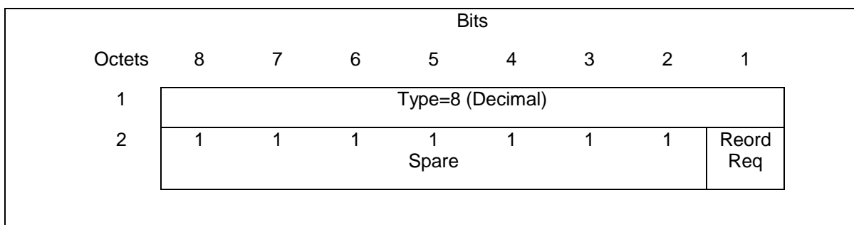
Figure 15: Reordering Required information element
