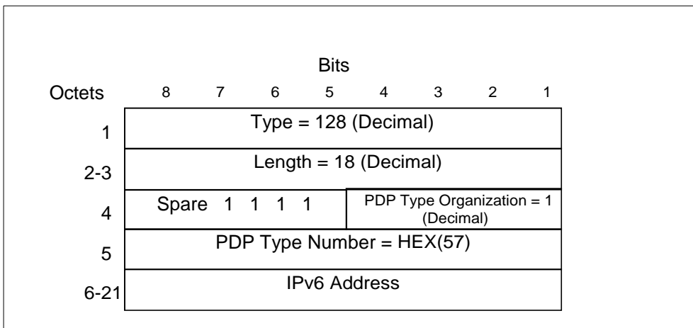
Figure 29: End User Address information element for IPv6
