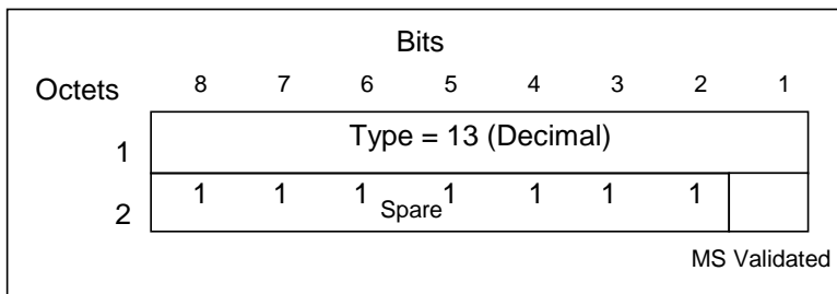
Figure 20: MS Validated information element
