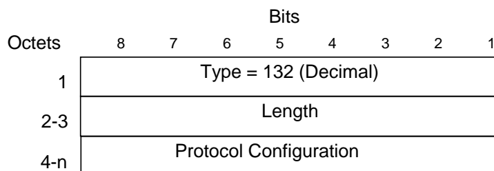
Figure 36: Protocol Configuration Options information element
