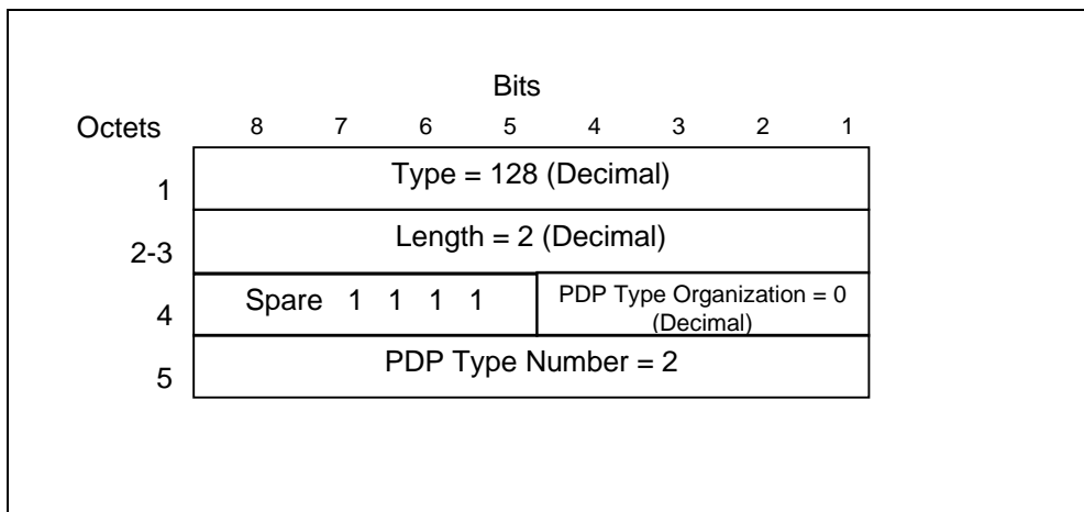
Figure 31: End User Address information element for PPP
