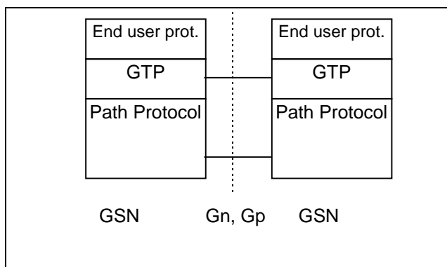
Figure 40: Transmission Plane - Protocol Stack
