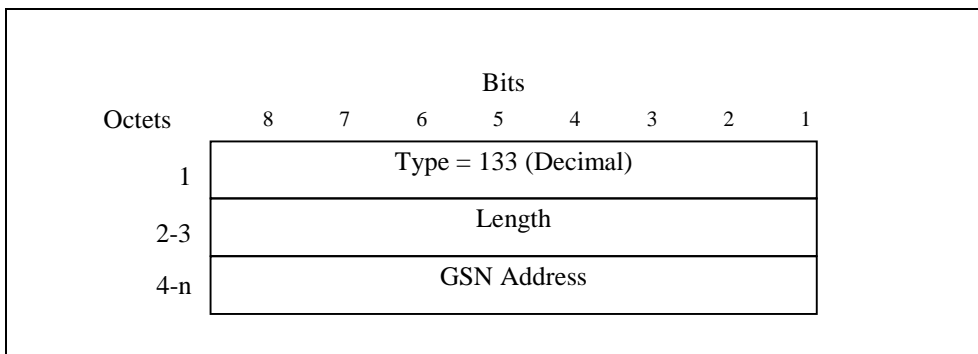
Figure 37: GSN Address information element
