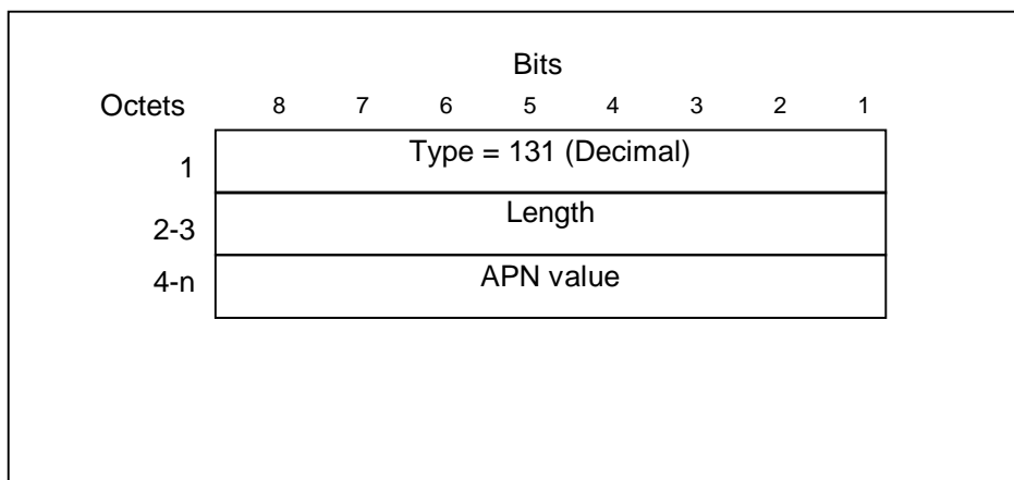
Figure 35: Access Point Name information element
