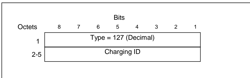
Figure 26: Charging ID information element
