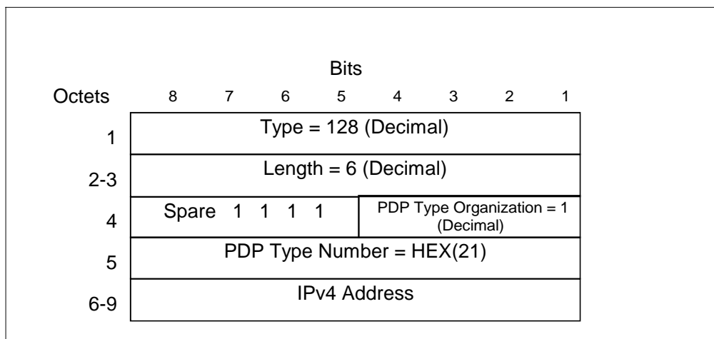
Figure 28: End User Address information element for IPv4
