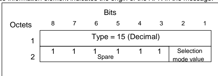
Figure 22: Selection mode information element
