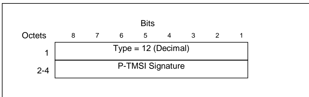
Figure 19: P-TMSI Signature information element
