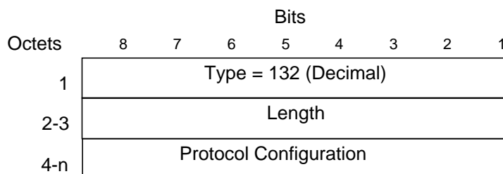
Figure 36: Protocol Configuration Options information element
