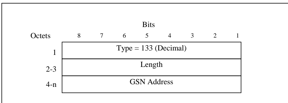
Figure 37: GSN Address information element
