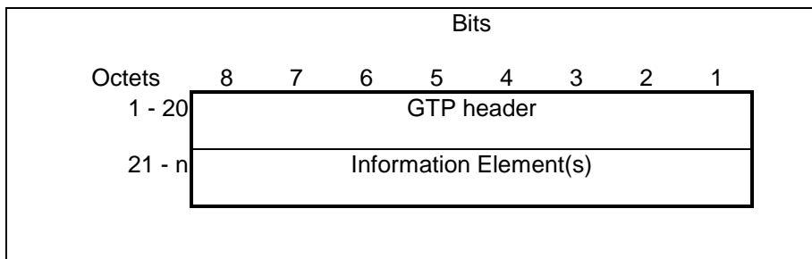
Figure 5: GTP header followed by subsequent Information Elements
