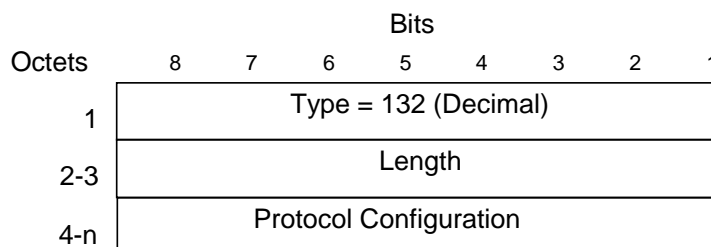
Figure 32: Protocol Configuration Options information element
