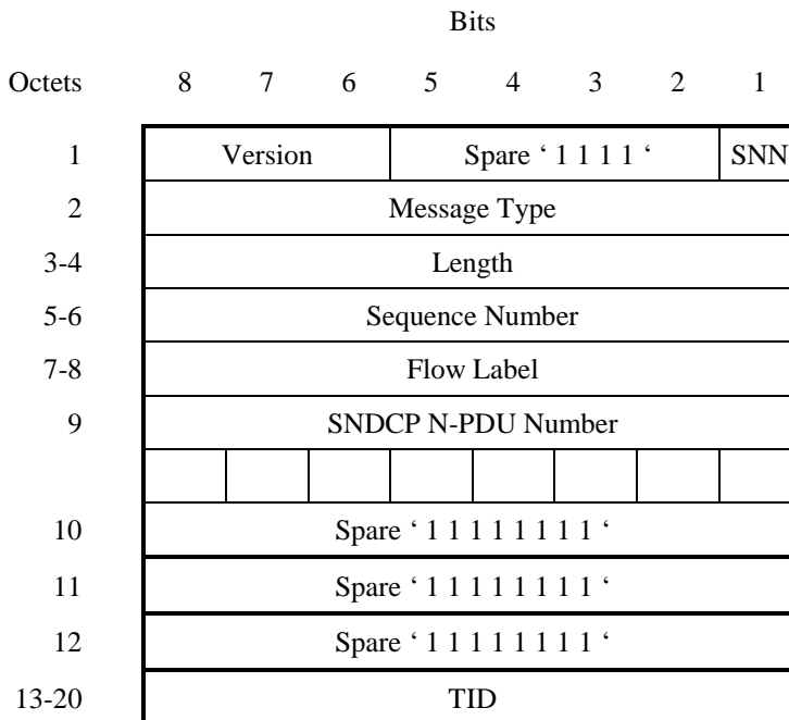
Figure 2: Outline of GTP header
