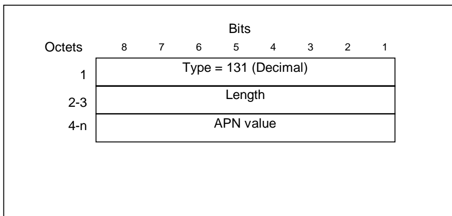
Figure 33: Access Point Name information element
