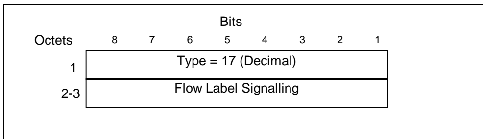
Figure 24: Flow Label Signalling information element
