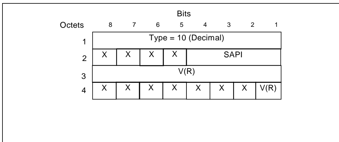
Figure 17: Receive State Variables information element
