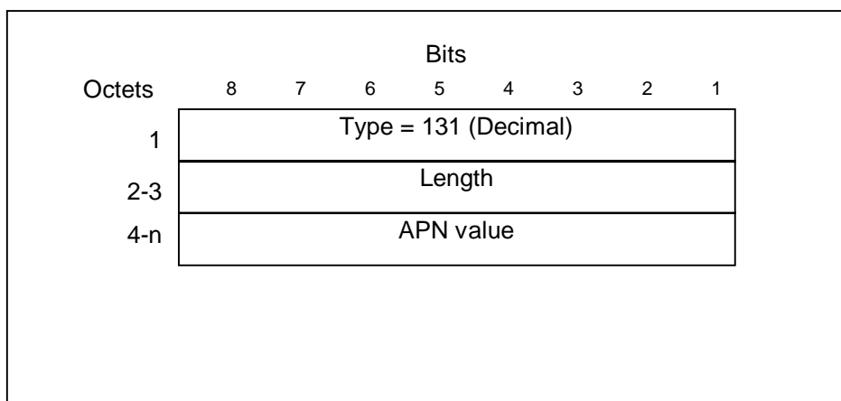
Figure 32: Access Point Name information element
