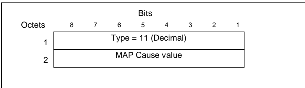
Figure 18: MAP Cause information element
