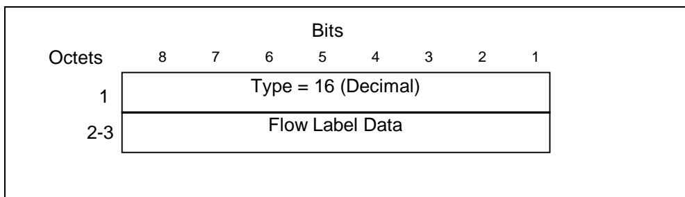
Figure 23: Flow Label Data information element
