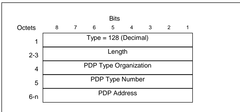
Figure 26: End User Address information element
