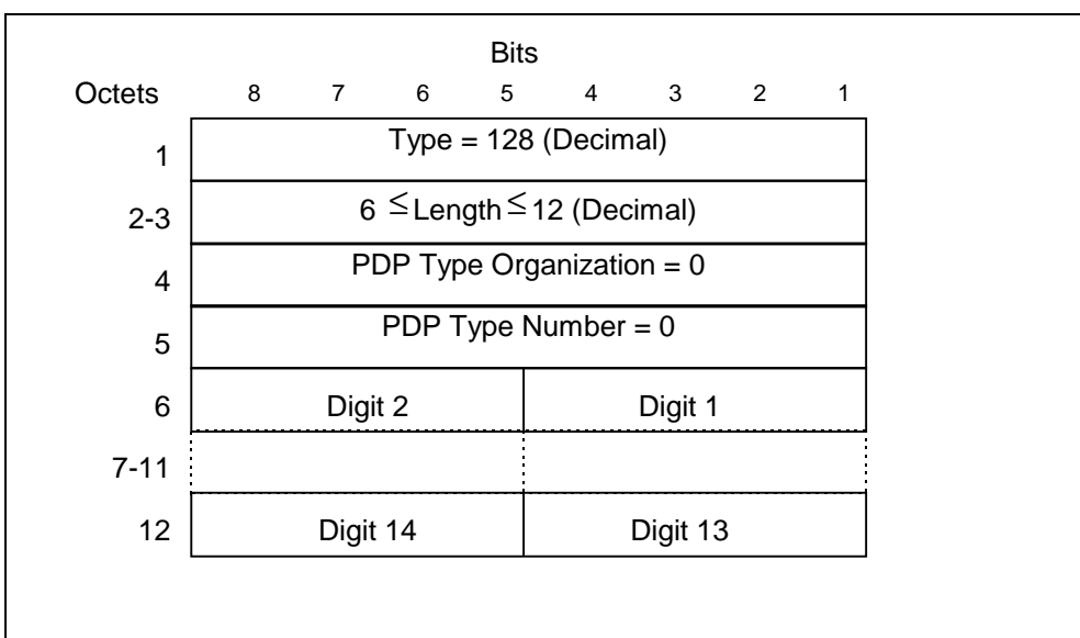
Figure 29: End User Address information element for X.25
