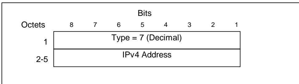
Figure 14: GSN Address information element
