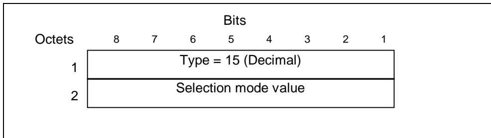
Figure 22: Selection mode information element
