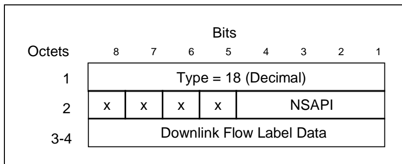
Figure 25: Flow Label Data II information element
