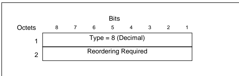
Figure 15: Reordering Required information element
