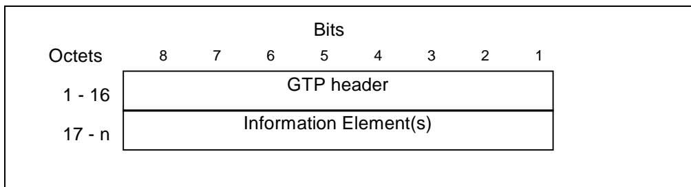
Figure 5: GTP header followed by subsequent Information Elements
