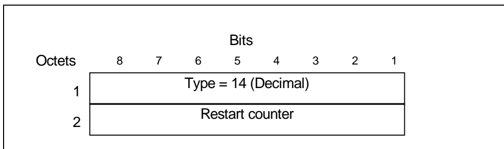
Figure 21: Restart counter information element
