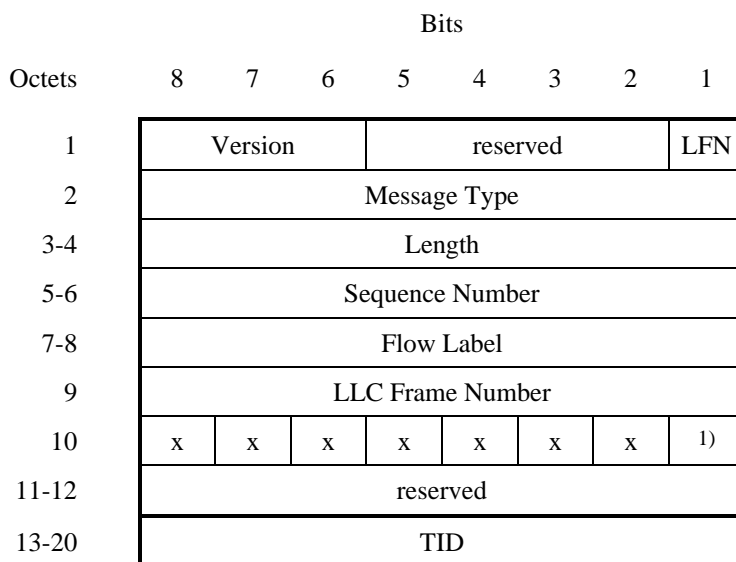
Figure 2: Outline of GTP header
