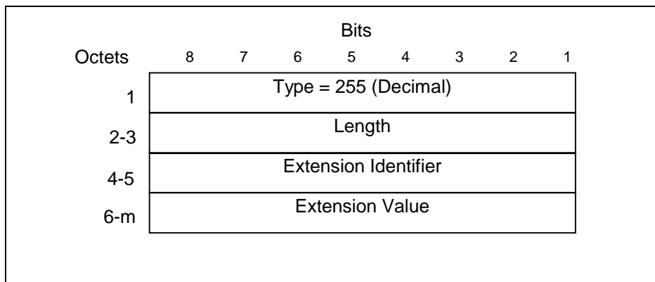
Figure 36: Private Extension information element
