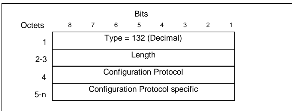
Figure 33: Protocol Configuration Options information element
