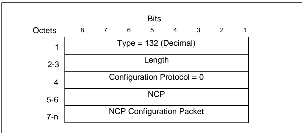
Figure 34: Protocol Configuration Options information element for PPP
