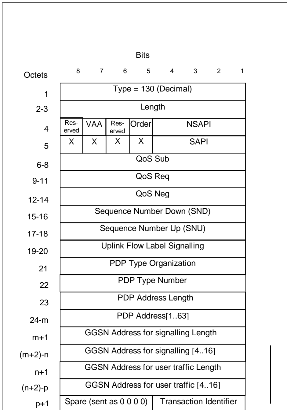
Figure 31: PDP Context information element
