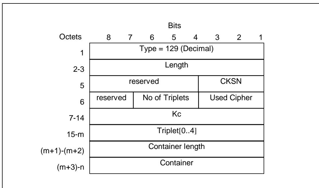
Figure 30: MM Context element
