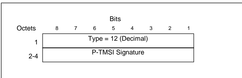
Figure 19: P-TMSI Signature information element
