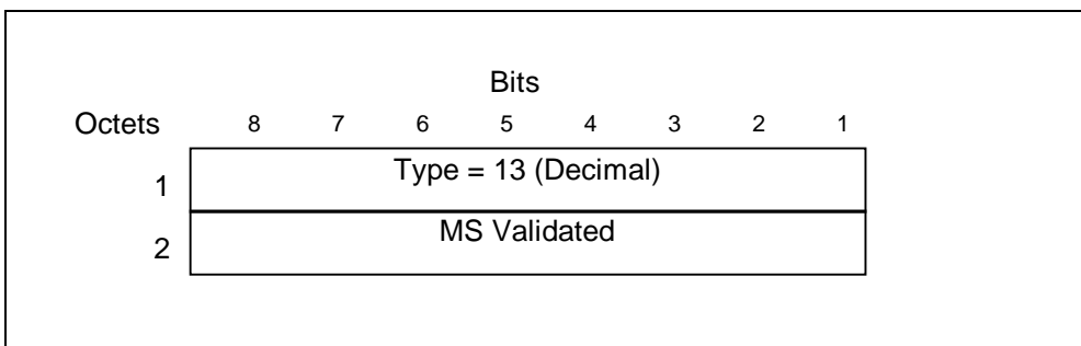
Figure 20: MS Validated information element
