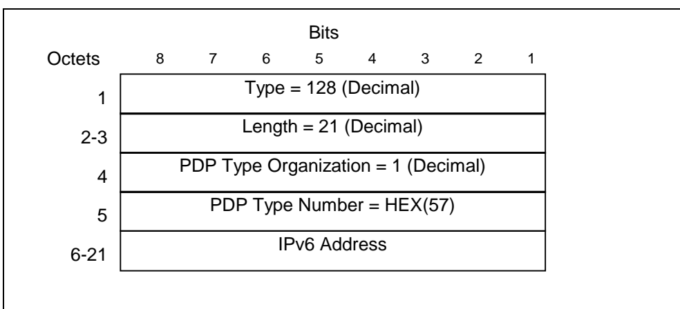
Figure 28: End User Address information element for IPv6
