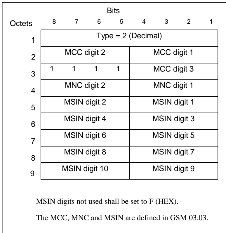
Figure 9: IMSI information element
