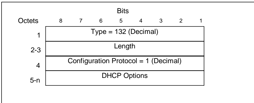
Figure 35: Protocol Configuration Options information element for DHCP
