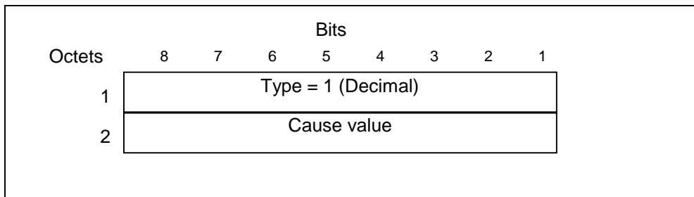
Figure 8: Cause information element
