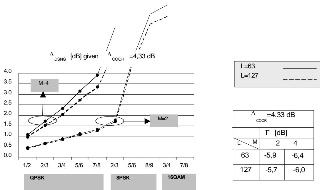
Figure D.3: 32 kbit/s co-ordination channels superimposed to DSNG. Example performance degradation of DSNG (R S = 6,666 Mbaud) interfered with by M co-ordination signals, with L = 63 and L = 127. The degradation of the co-ordination channels has been assumed to be Δ COOR = 4,33 dB.
