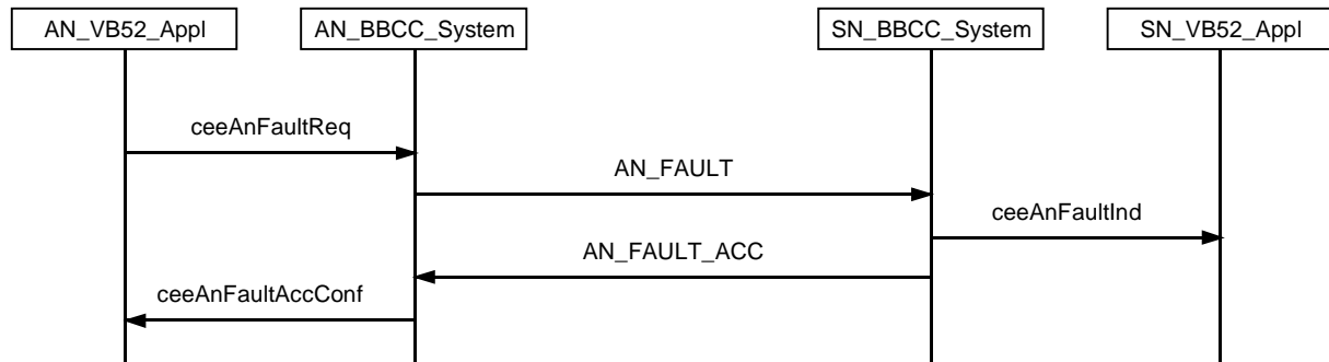
Figure 30: AN fault procedure
