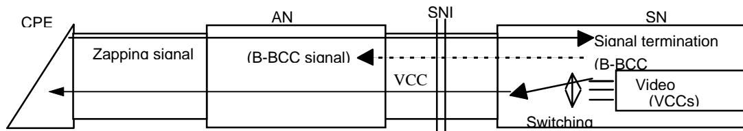
Figure F.2: Architecture 2: Support of SVB with video signal switching function in the SN
