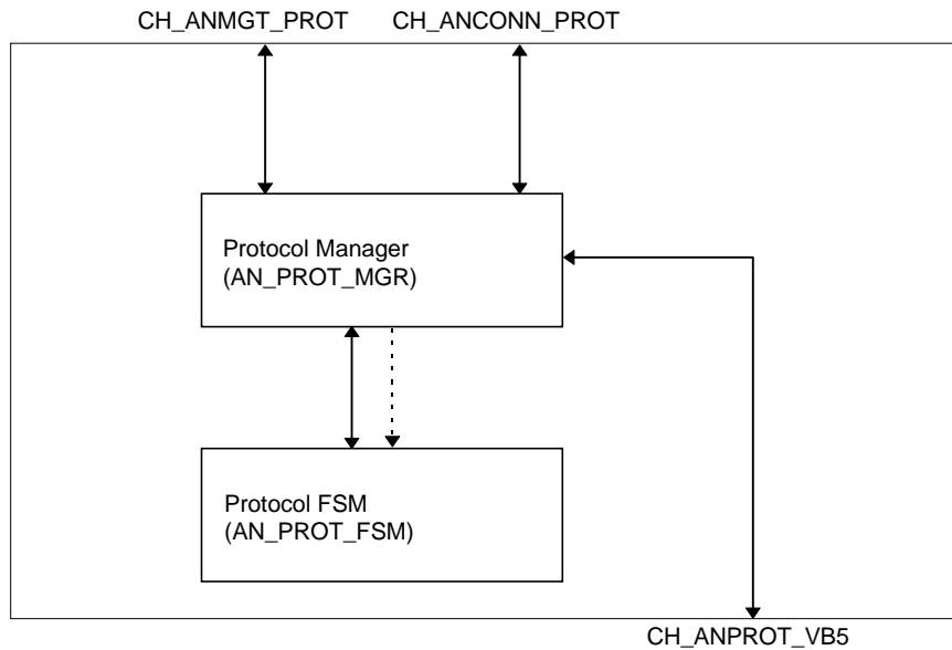
Figure 19: AN B-BCC protocol block
