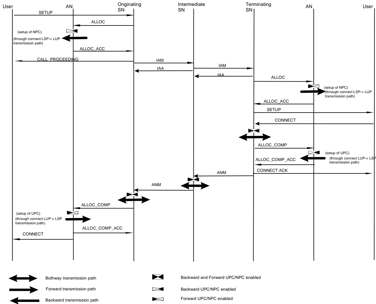
Figure D.1: Connection is not susceptible to information/speech clipping
