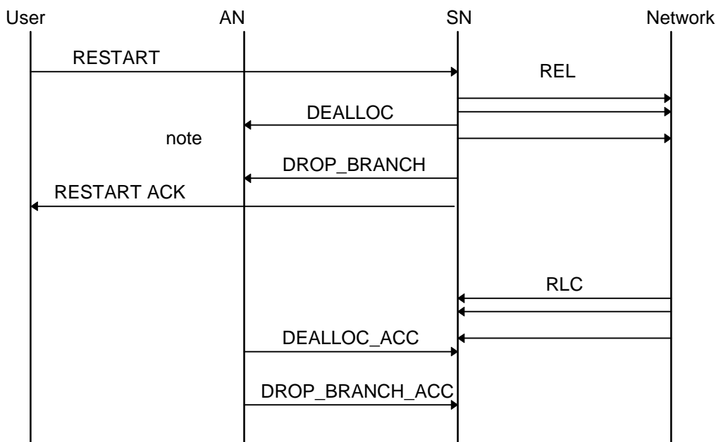
Figure C.12: DSS2 restart
