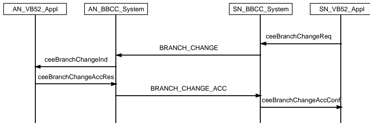
Figure F.5: Change branch procedure
