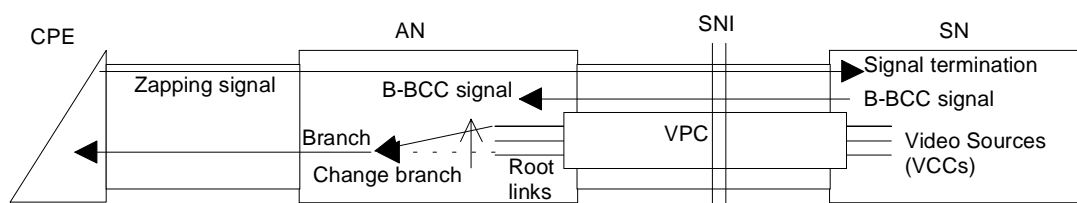
Figure F.3: Change of a branch in the AN
