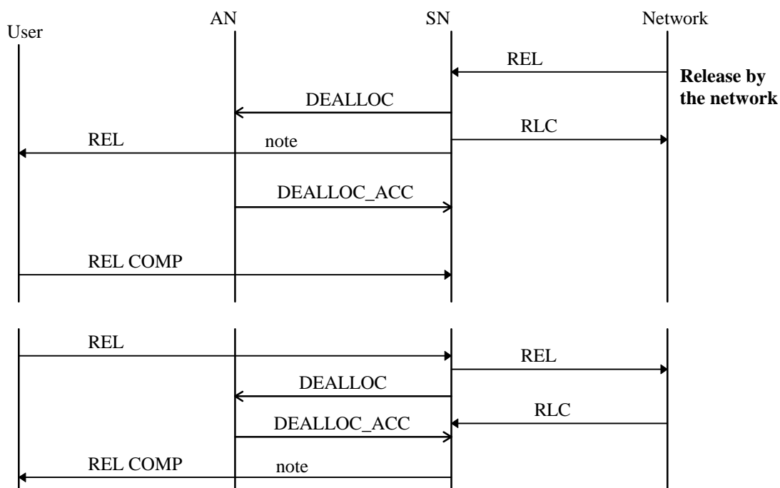
Figure C.9: Connection release
