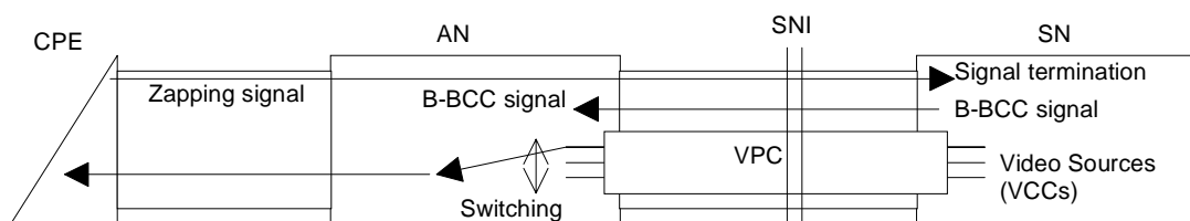
Figure F.1: SDV architecture that related VB5.2 reference point
