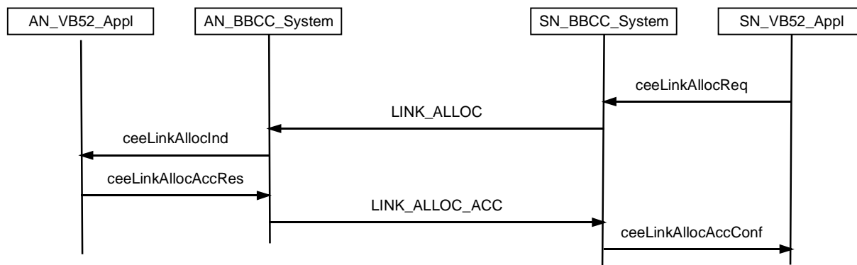
Figure F.4: Link establishment procedure
