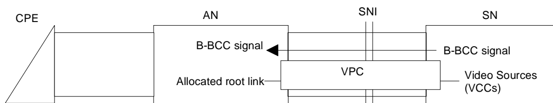
Figure F.2: Root link allocation at VB5.2 reference point
