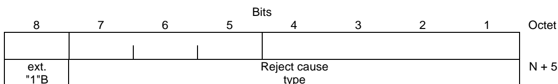
Figure 38: Reject cause information element coding
