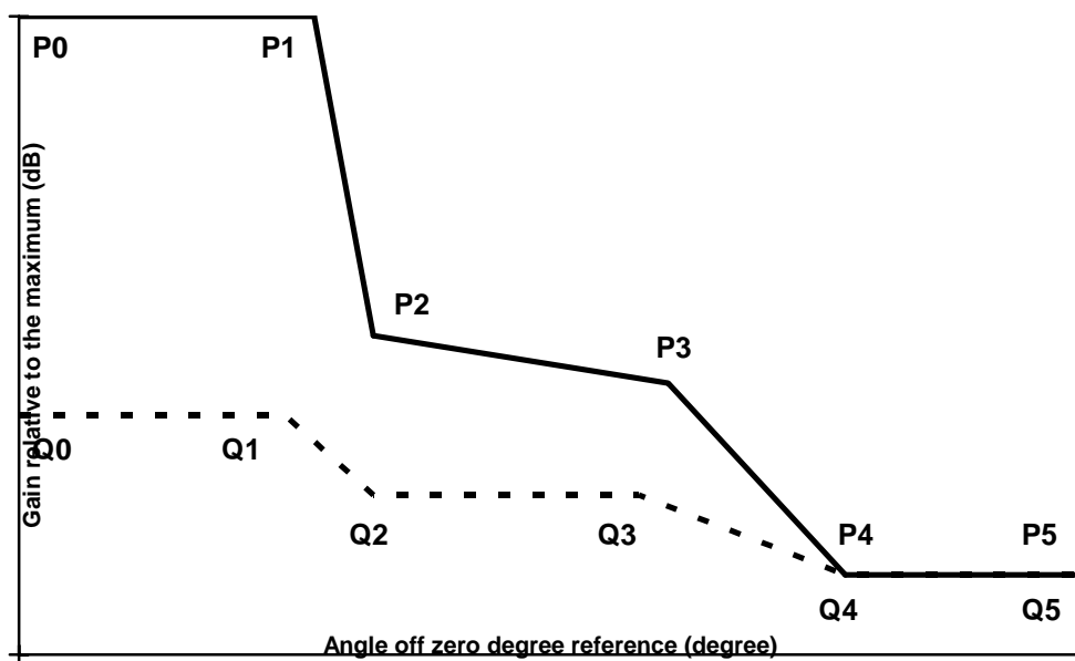
Figure 5: Normalized CS4 sector antenna template for azimuth
