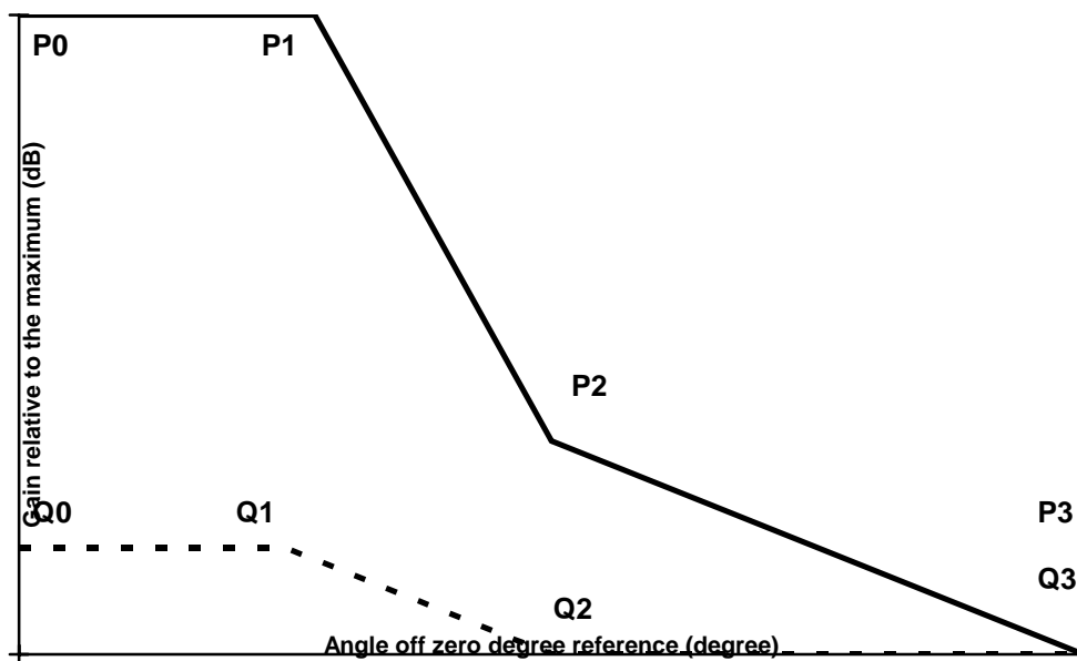
Figure 4: Normalized CS3 sector antenna template for azimuth
