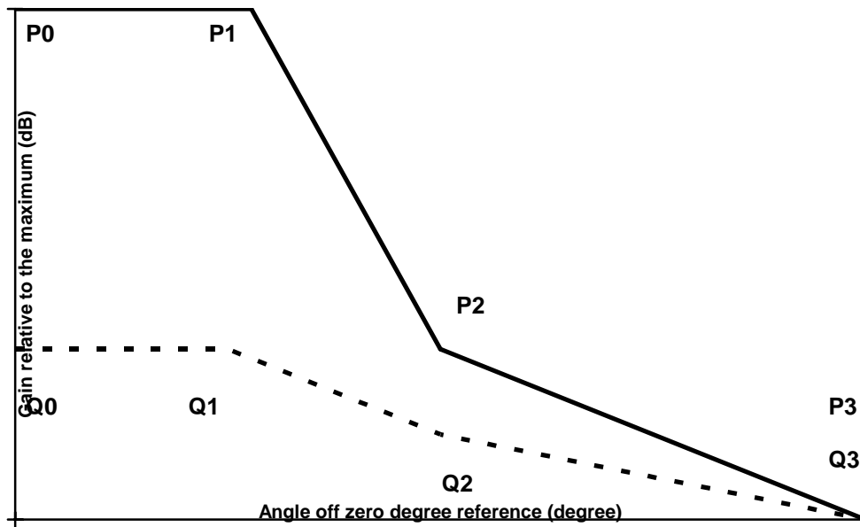
Figure 3: Normalized CS2 sector antenna template for azimuth
