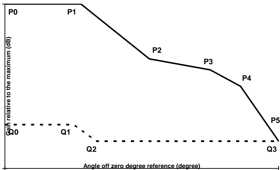
Figure 2: Normalized CS1 sector antenna template for azimuth
