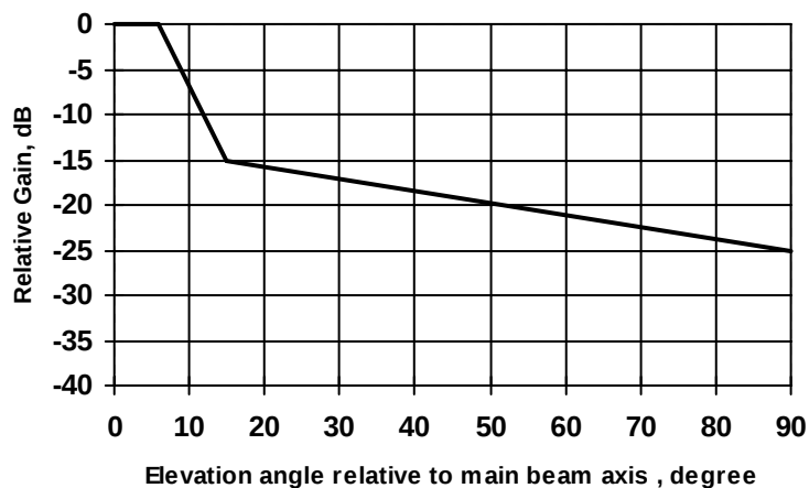
Figure 6: Symmetric CS antenna co-polar elevation RPE
