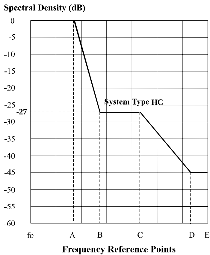
Figure 3: Spectrum mask, type HC ( f_o = actual carrier frequency)
