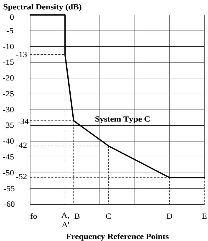
Figure 2: Spectrum mask, type C ( f_o = actual carrier frequency)
