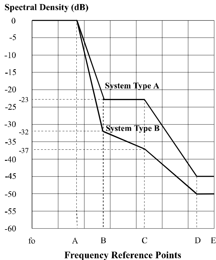
Figure 1: Spectrum masks, types A and B (fo = actual carrier frequency)
