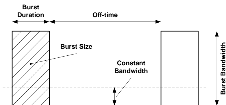
Figure 7: Burst parameters
