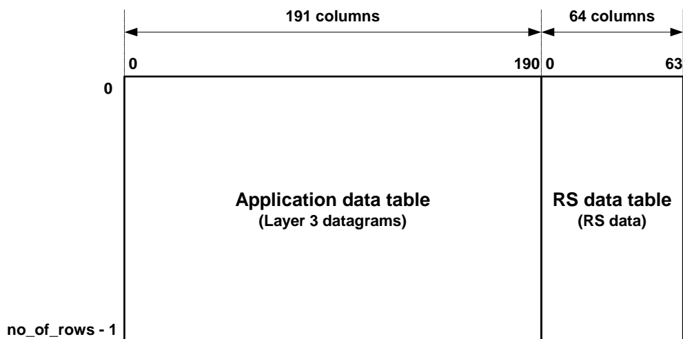
Figure 13: The structure of the MPE-FEC Frame
