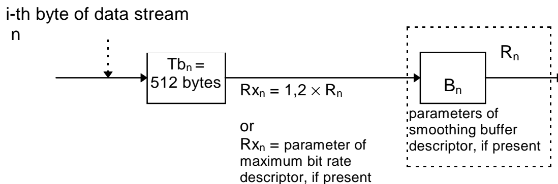
Figure 4: Data service decoder model
