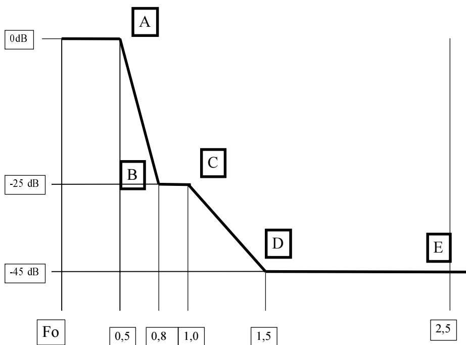
Figure 4: FH-CDMA spectrum mask normalized for channel spacing
