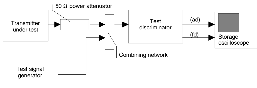
Figure 3: Measurement arrangement
