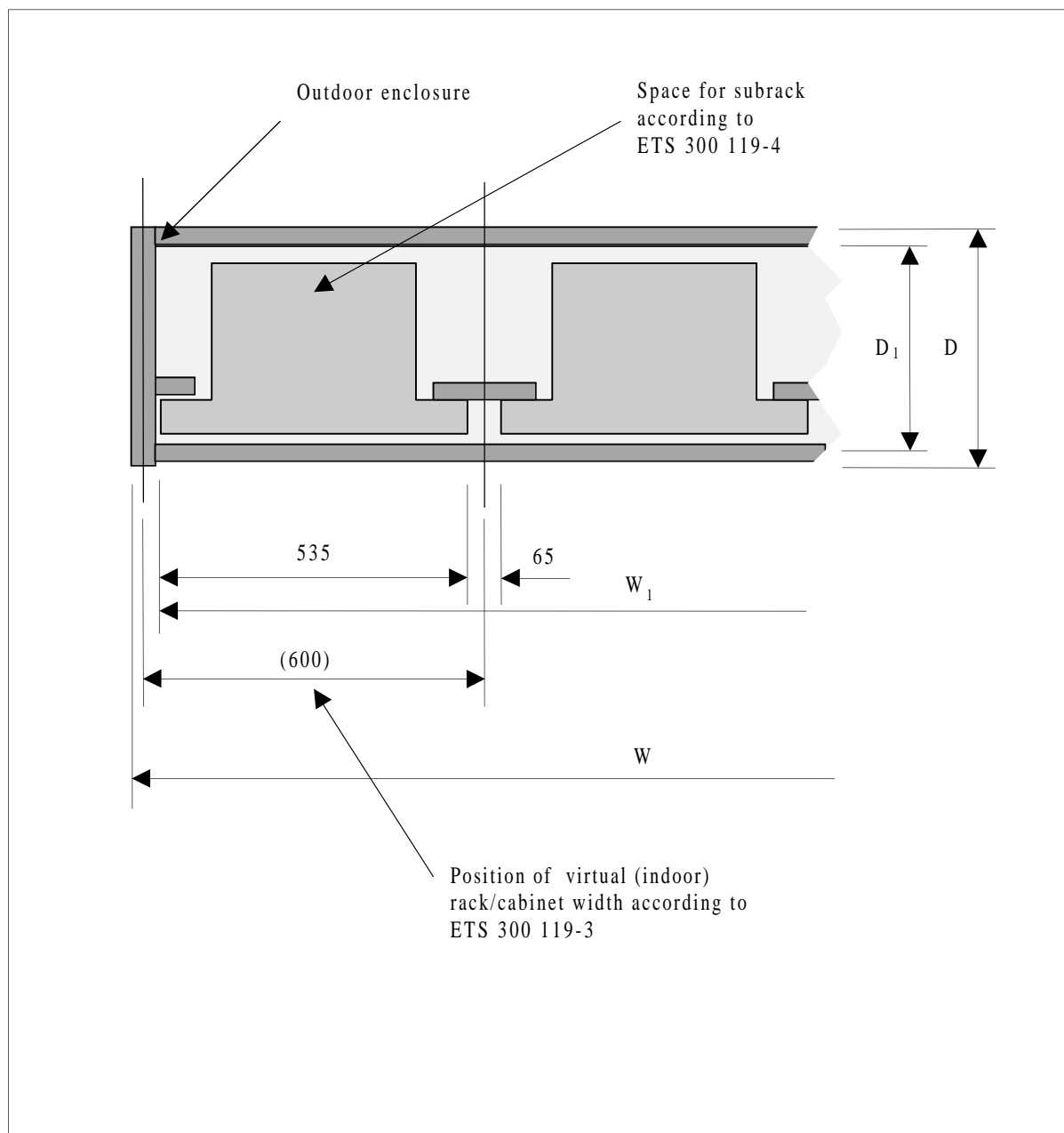
Figure A.2: Co-ordination dimensions for unequipped outdoor enclosures / subrack deployment
