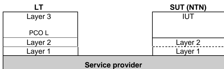
Figure 1: Remote test method
