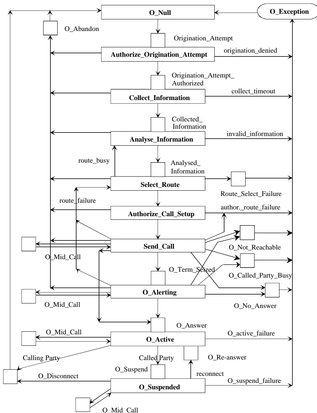
Figure 4-1: Originating BCSM for CS2
