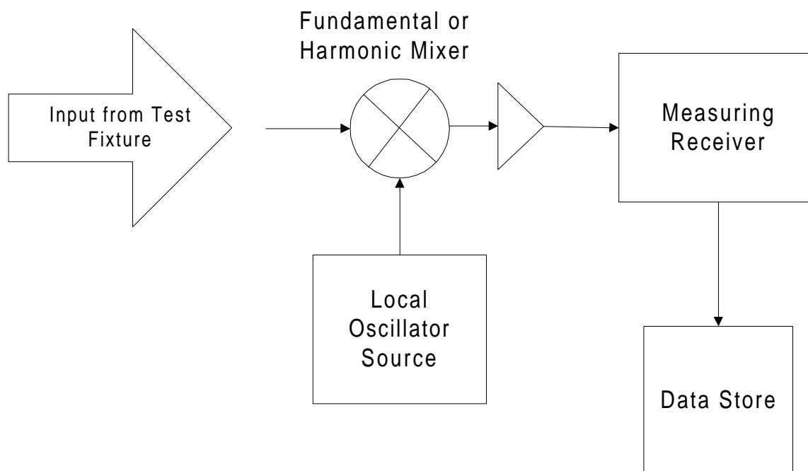
Figure 6: Test equipment for measuring the modulation waveform
