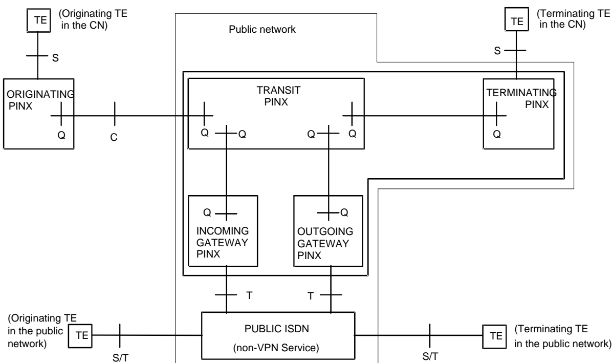
Figure A.3: Transit and terminating functions provided by the public network
