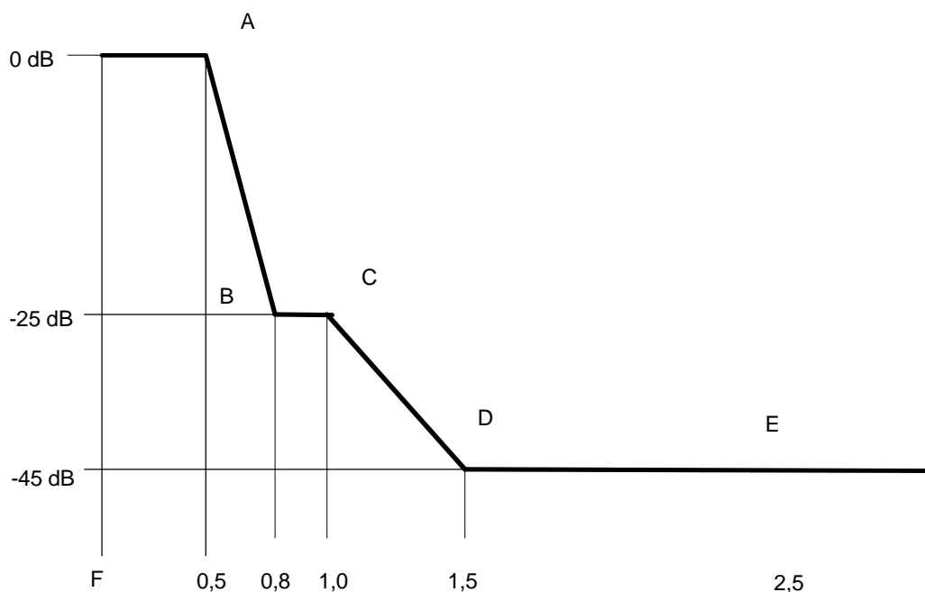
Figure 3: DS-CDMA spectrum mask normalized to channel spacing
