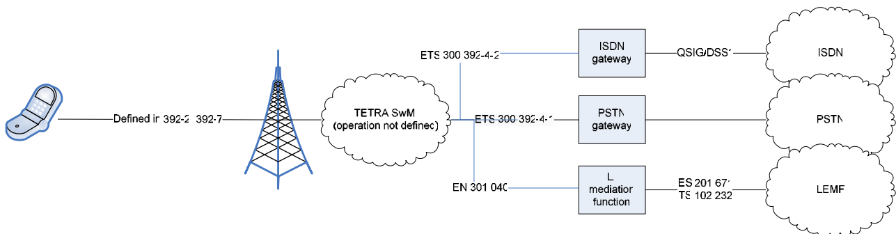
Figure 1: Model of TETRA interception
