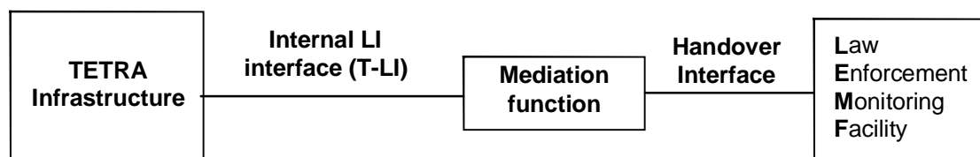
Figure 1: General reference model of lawful interception from user perspective
