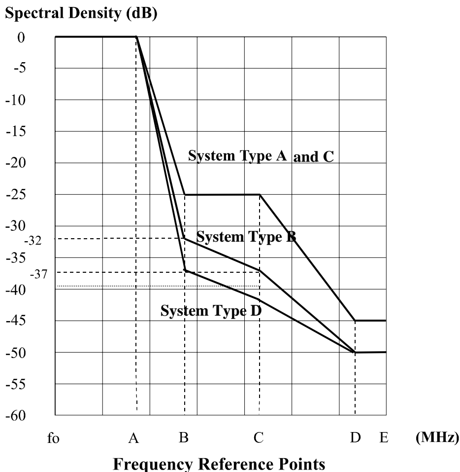
Figure 3: Power spectrum masks ( f_0 = actual carrier frequency)
