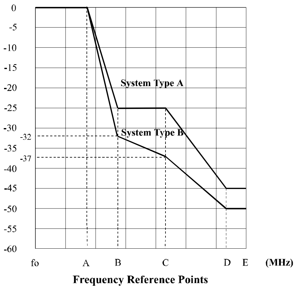
Figure 3: Power spectrum masks (fo = actual carrier frequency)
