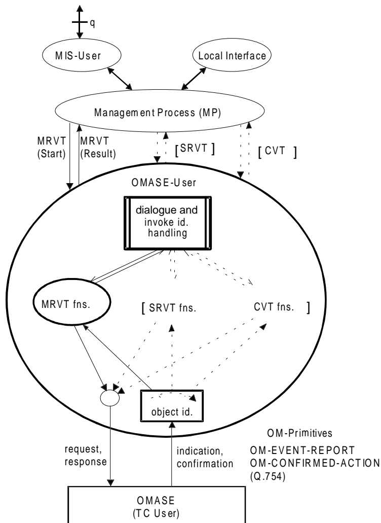
Figure A.1/Q.753: Detailed model of the OMASE-User and its interfaces
