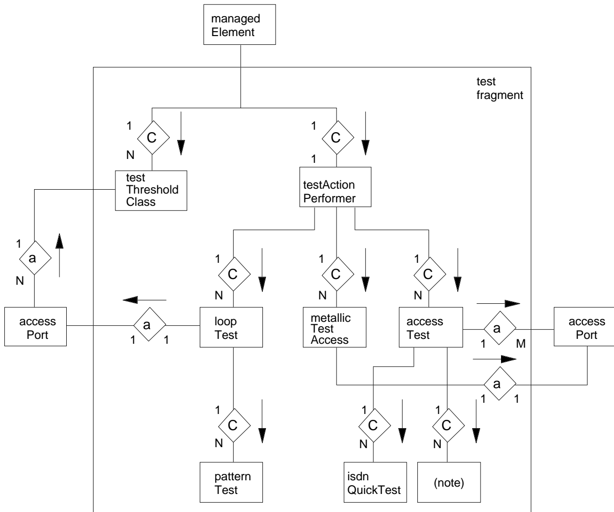
Figure 2: Entity relationship diagram - test fragment
