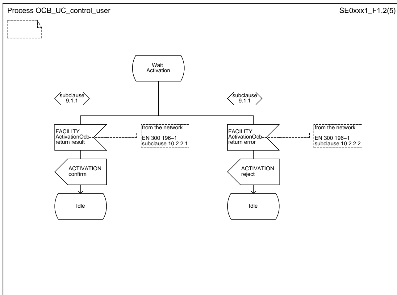
Figure 1 (sheet 2 of 5): OCB-UC management procedures - user side
