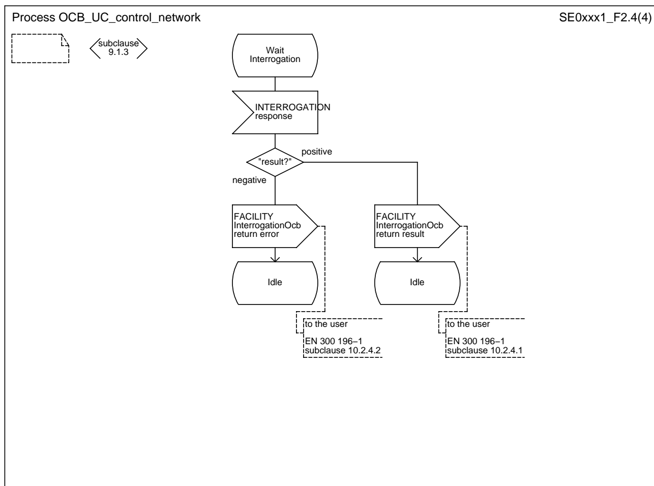
Figure 2 (sheet 4 of 4): OCB-UC management procedures - network side
