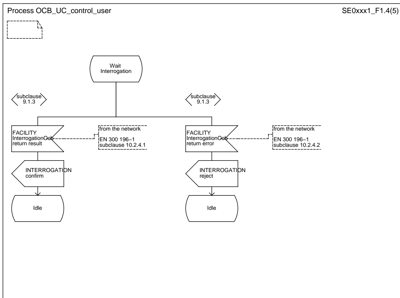
Figure 1 (sheet 4 of 5): OCB-UC management procedures - user side
