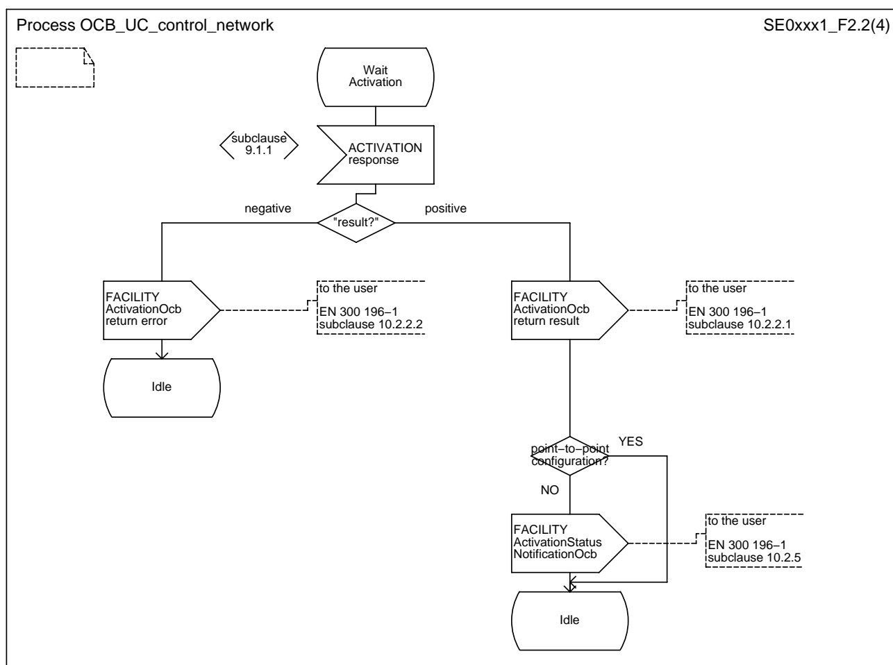
Figure 2 (sheet 2 of 4): OCB-UC management procedures - network side
