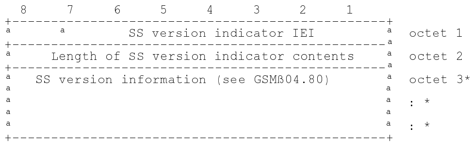
Figure 10.5.113/GSM 04.08
