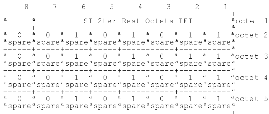
Figure 10.5.64/GSM 04.08 SI 2ter Rest Octets information element
