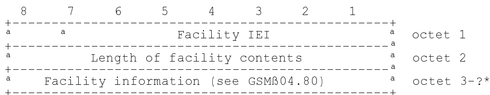
Figure 10.5.101/GSM 04.08
