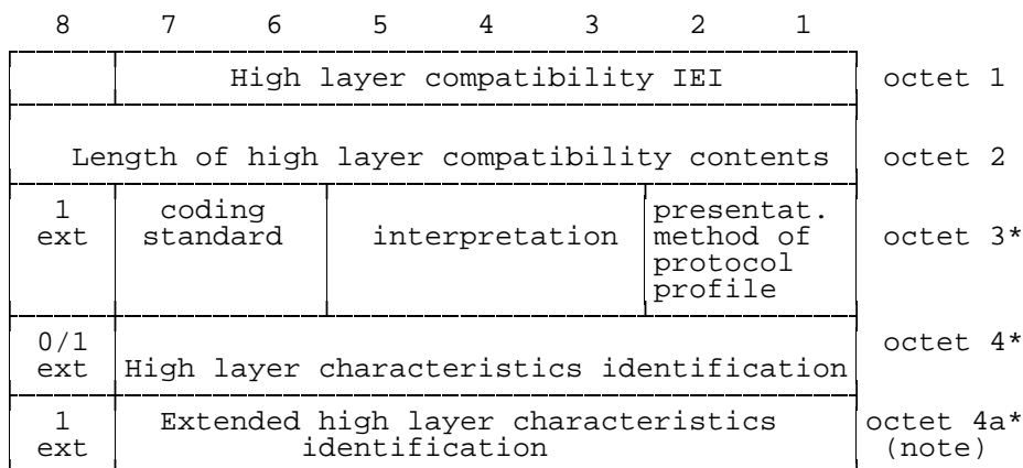
Figure 10.83/GSM 04.08: High layer compatibility information element
