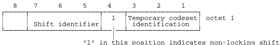
Figure 10.69/GSM 04.08: Non-locking shift element
