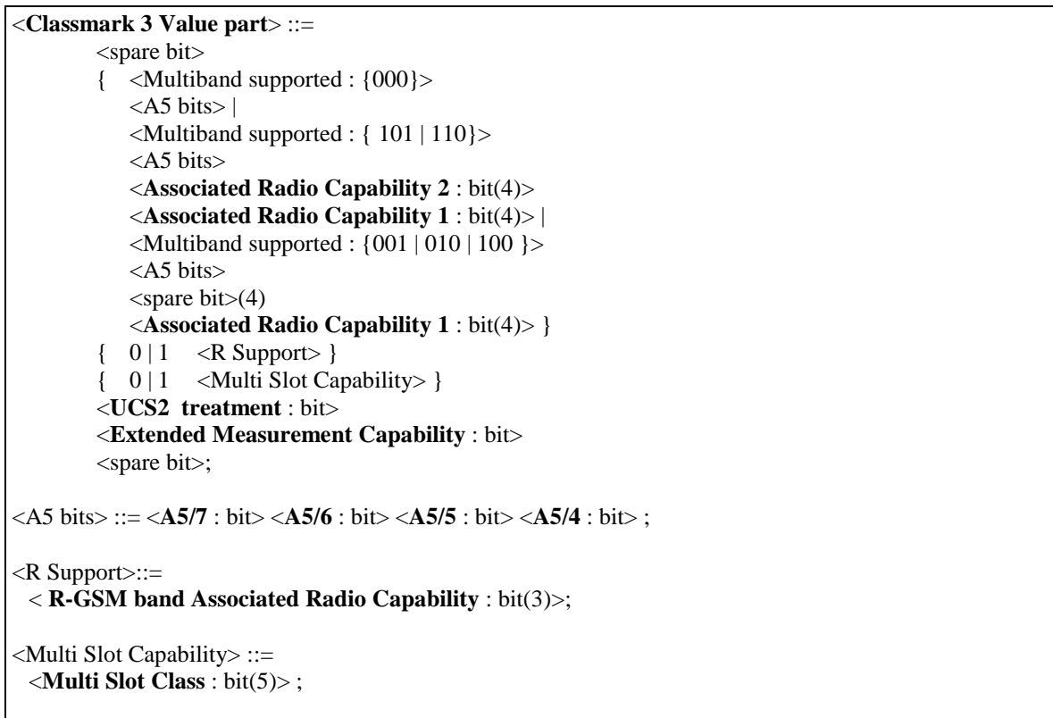
Figure 10.8/GSM 04.08: Mobile Station Classmark 3 information element
