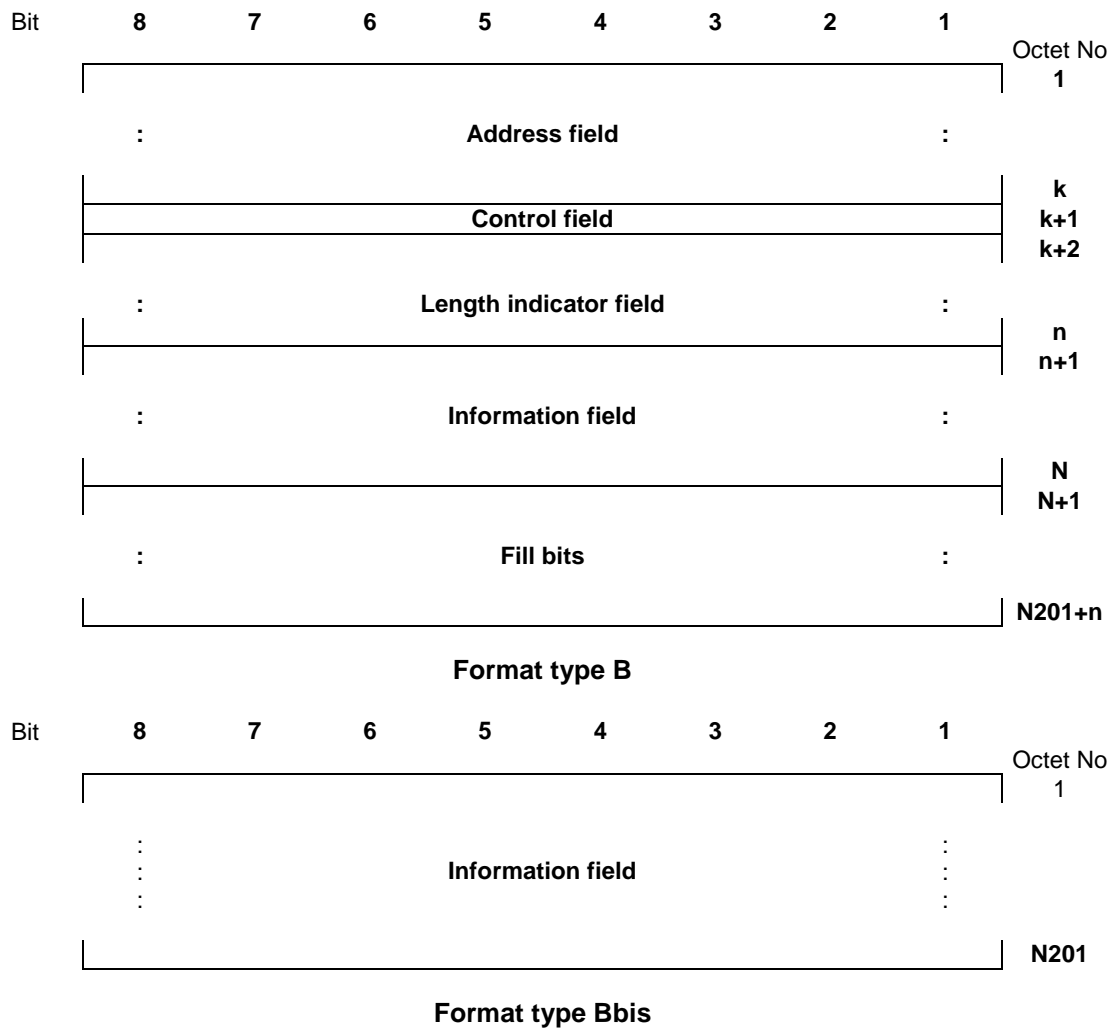
Figure 1/GSM 04.06 (sheet 2 of 3): General frame formats
