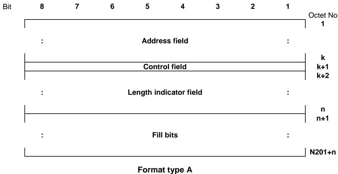
Figure 1/GSM 04.06 (sheet 1 of 3): General frame formats
