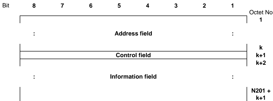
Figure 1/GSM 04.06 (sheet 2 of 3): General frame formats
