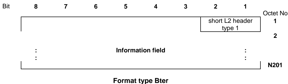
Figure 1/GSM 04.06 (sheet 3 of 3): General frame formats
