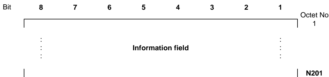
Figure 1/GSM 04.06 (sheet 2 of 3): General frame formats
