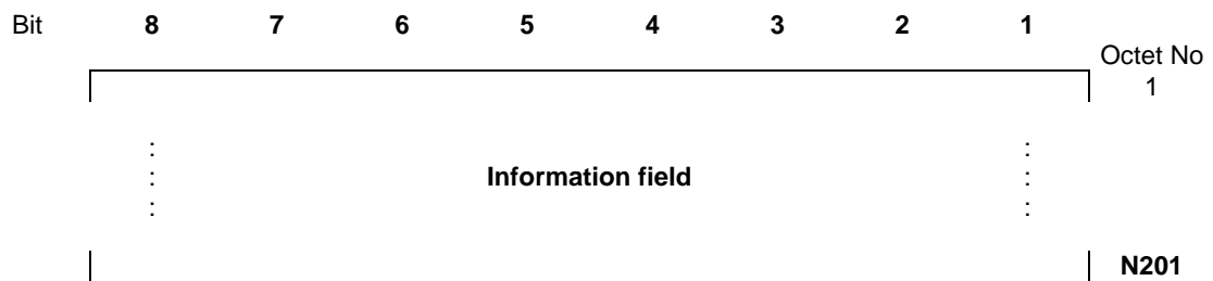
Figure 1/GSM 04.06 (sheet 2 of 3): General frame formats
