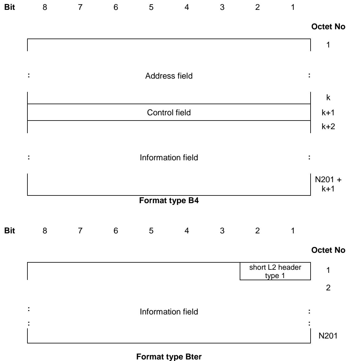
Figure 1/GSM 04.06 (sheet 3 of 3): General frame formats
