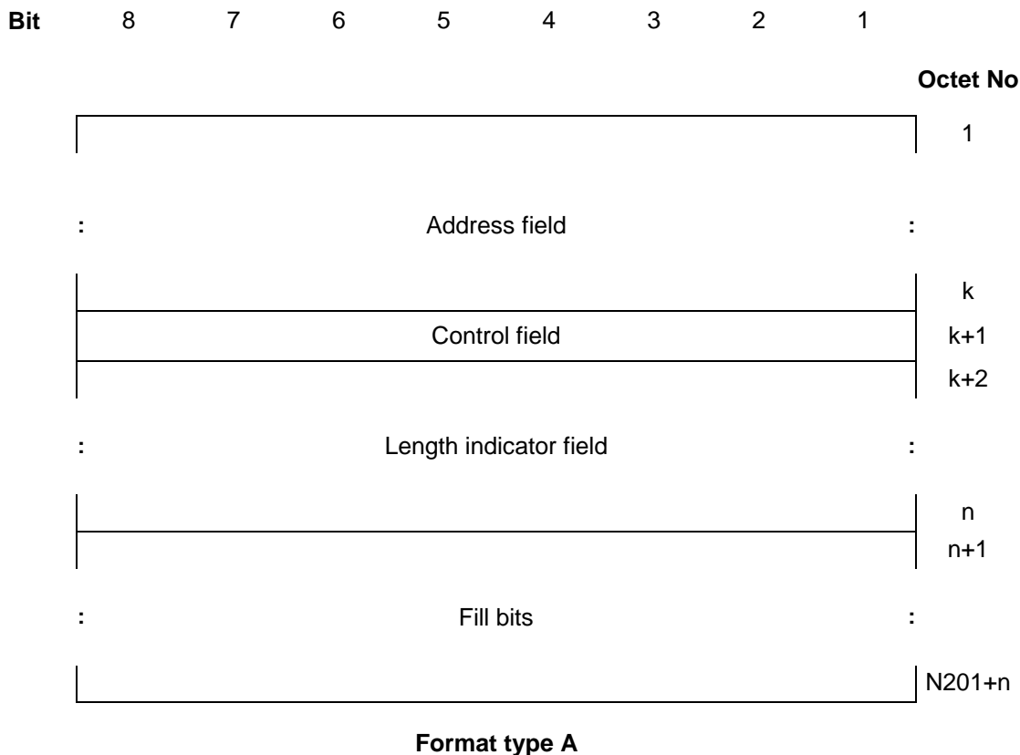
Figure 1/GSM 04.06 (sheet 1 of 3): General frame formats
