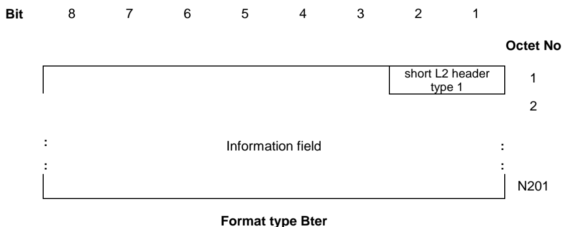
Figure 1/GSM 04.06 (sheet 3 of 3): General frame formats
