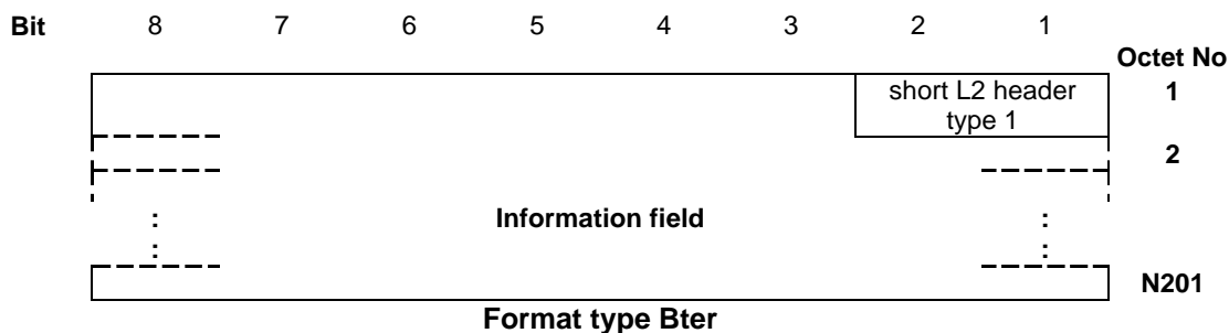
Figure 1/GSM 04.06 (sheet 3 of 3): General frame formats
