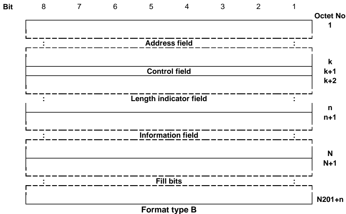
Figure 1/GSM 04.06 (sheet 1 of 3): General frame formats
