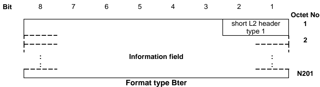
Figure 1/GSM 04.06 (sheet 3 of 3): General frame formats
