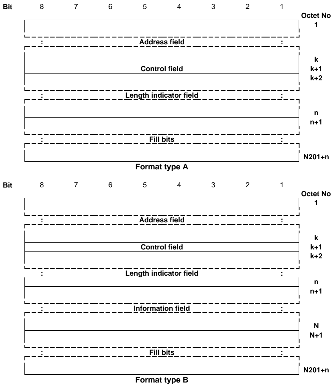
Figure 1/GSM 04.06 (sheet 1 of 3): General frame formats
