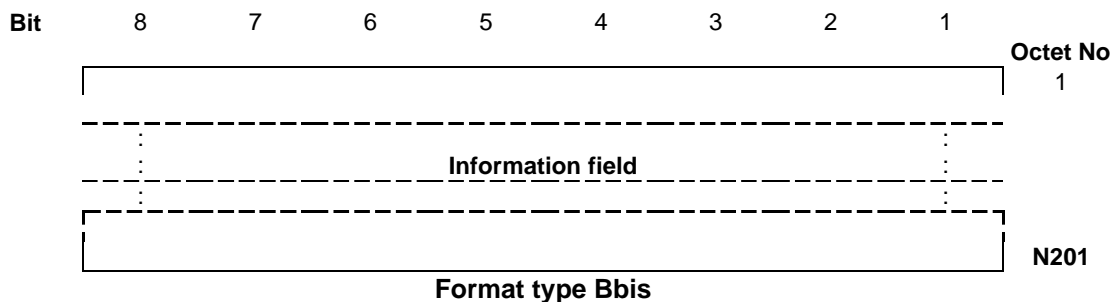
Figure 1/GSM 04.06 (sheet 2 of 3): General frame formats
