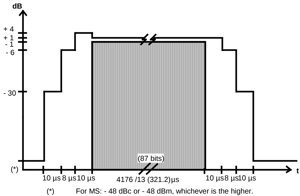
PCS 1 900 MS Access Burst Time Mask
