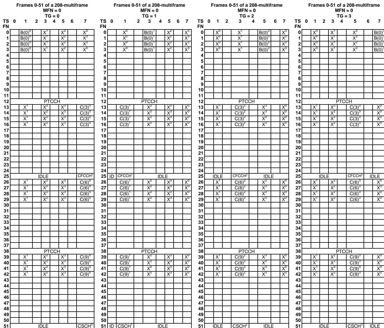
Figure D.1: COMPACT downlink 52-multiframe structure using 4 time groups for nominal cells (based on an assignment of 1 CPBCH and 3 CPCCCHs with NIB_CPBCH_0 = NIB_CCCH_1 = NIB_CCCH_2 = NIB_CCCH_3 = 4). NIB_CCCH is not broadcast for serving cell time group.
