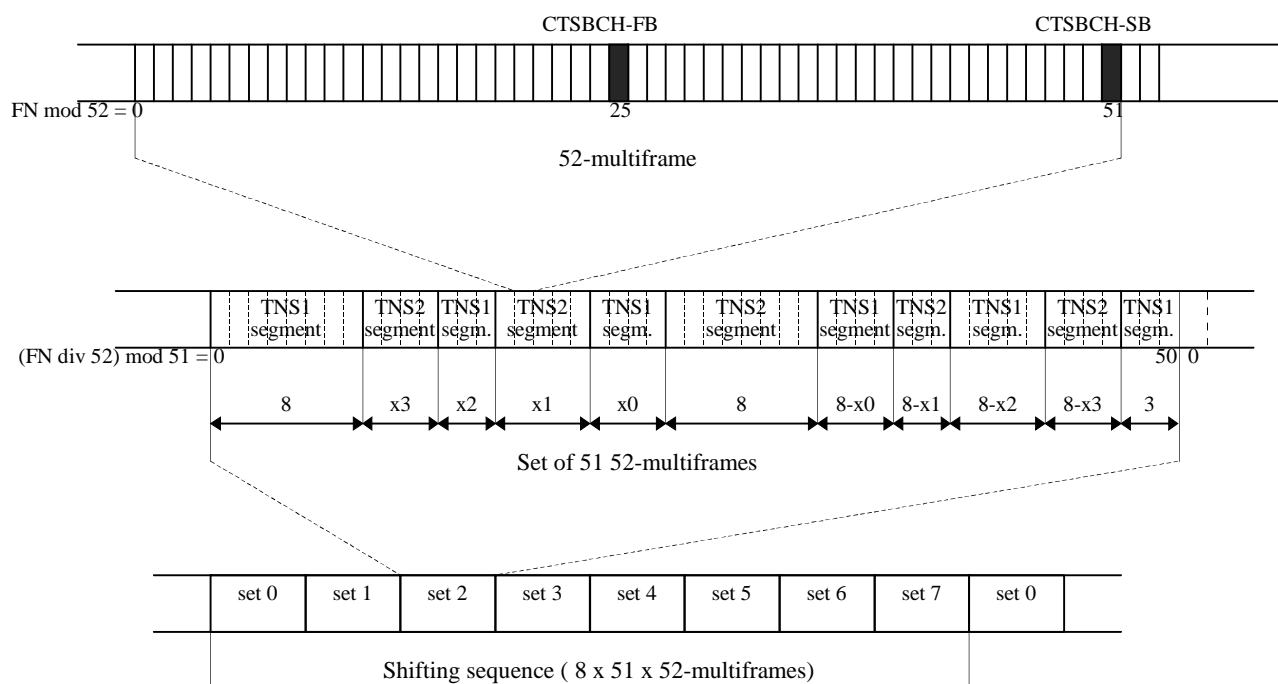
Figure 1 (subclause 6.3.3): Structure of timeslot shifting sequence
