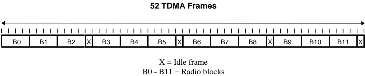
Figure 9 : 52- multiframe for PDCHs -
