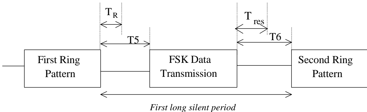
Figure 6: Data transmission during ringing
