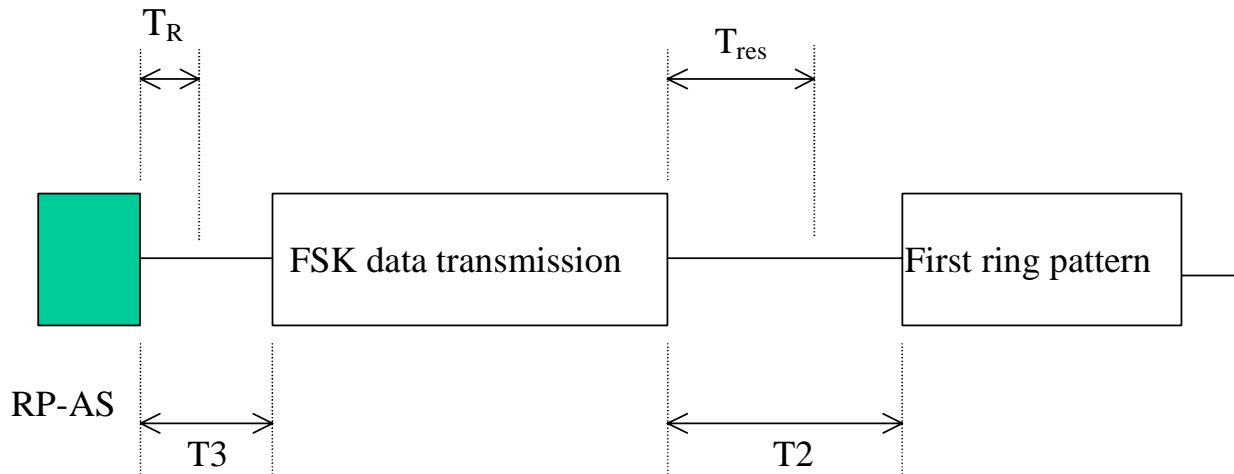
Figure 4: RP-AS alerting signal
