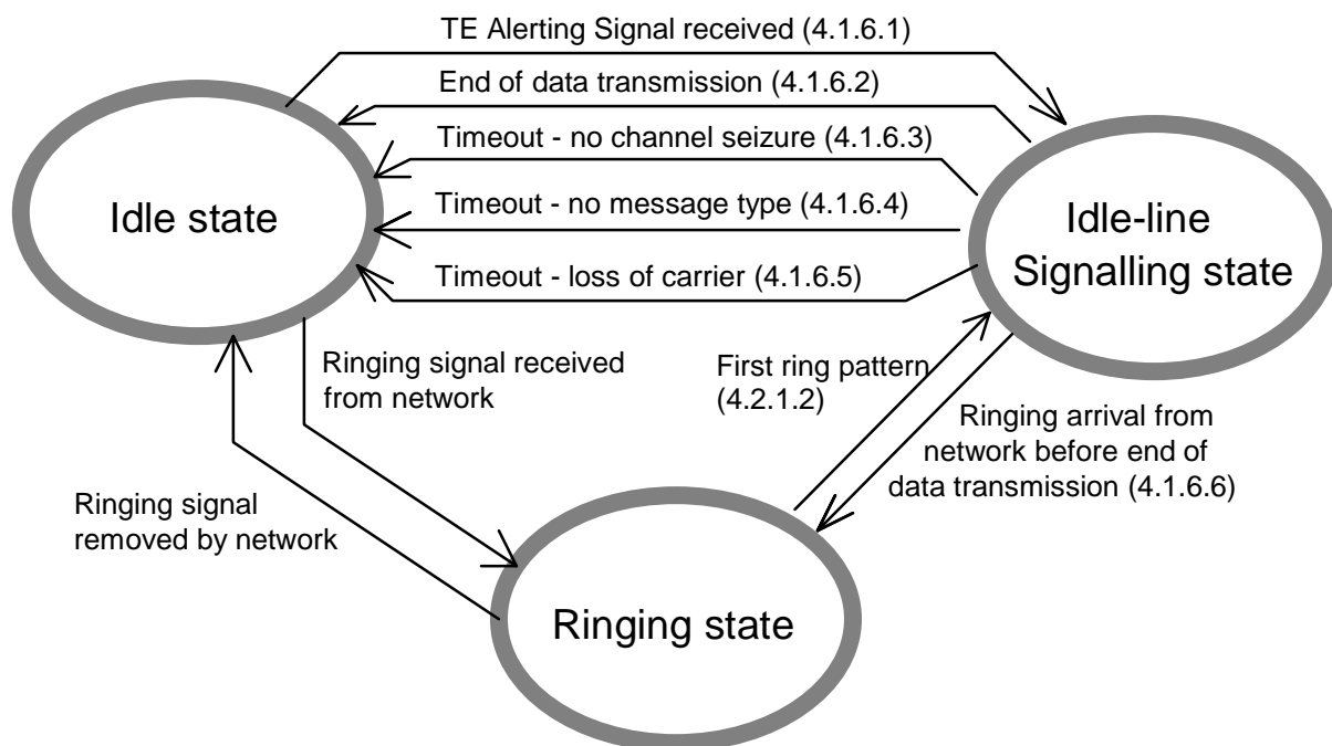
Figure 1: State diagram
