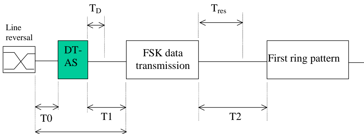
Figure 5: LR + DT-AS alerting signal
