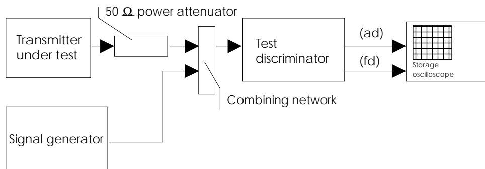
Figure 3: Measurement arrangement
