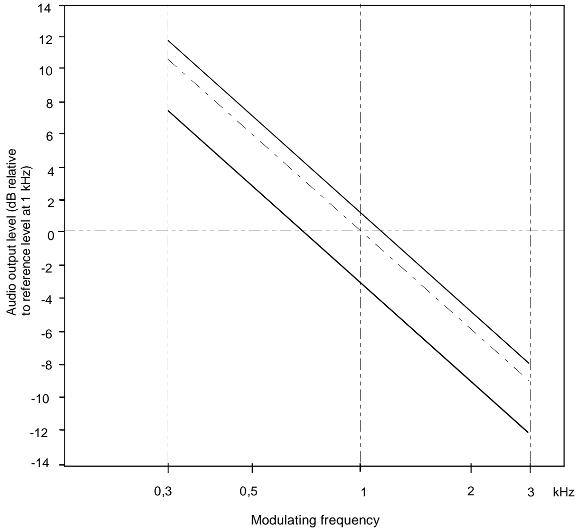
Figure 5: Audio frequency response
