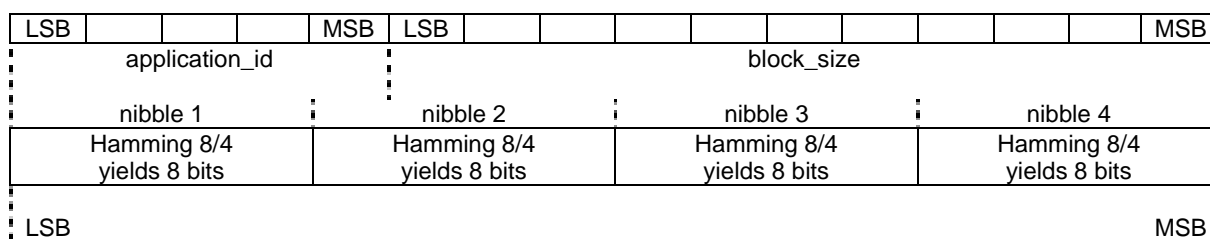
Figure A.2: Structure Header as defined in EN 300 708 [1]
