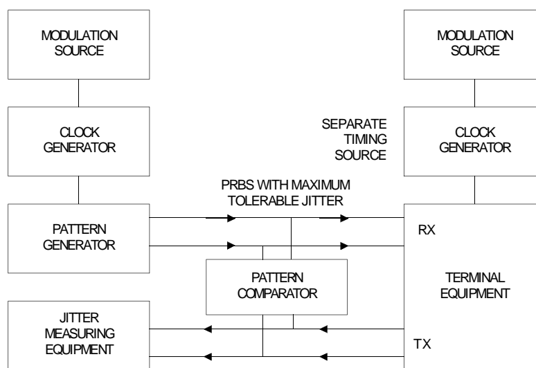
Figure A.7: Jitter measurement
