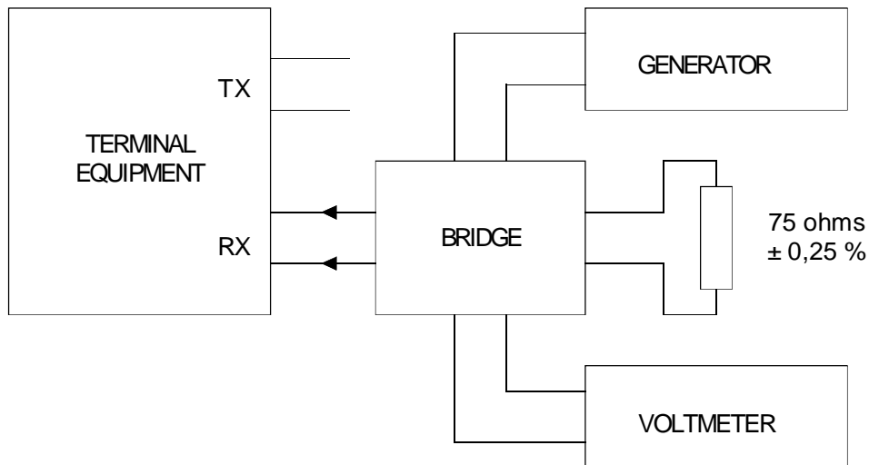
Figure A.5: Return loss at input port
