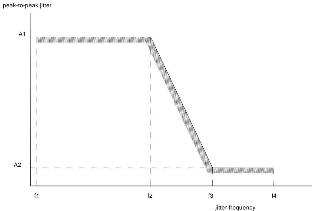
Figure 3: Input jitter tolerance
